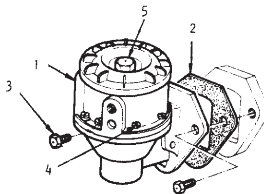
BOMBA "GM-DFV"
