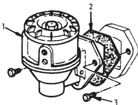
BOMBA "DFV"
